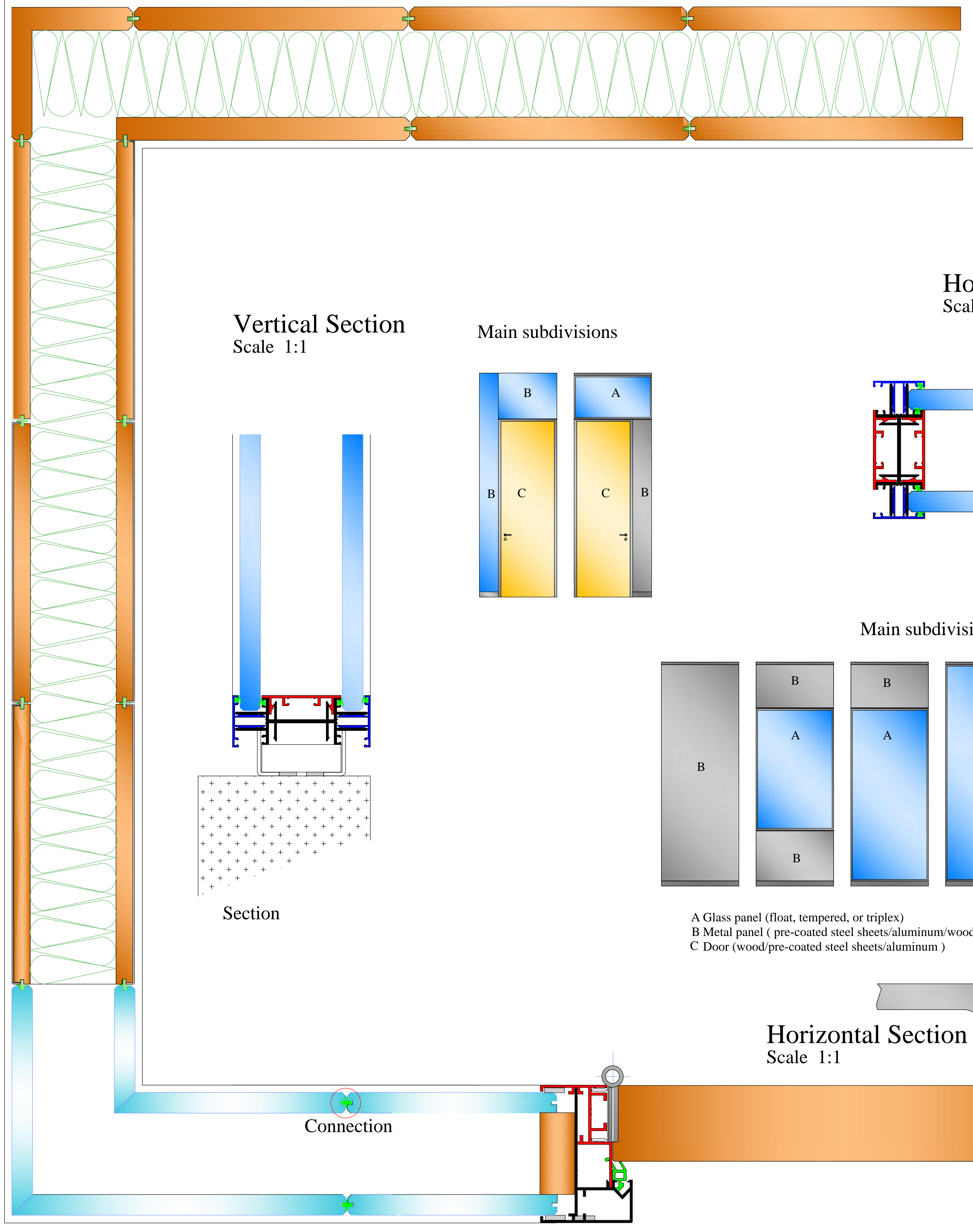
Corner Connection
