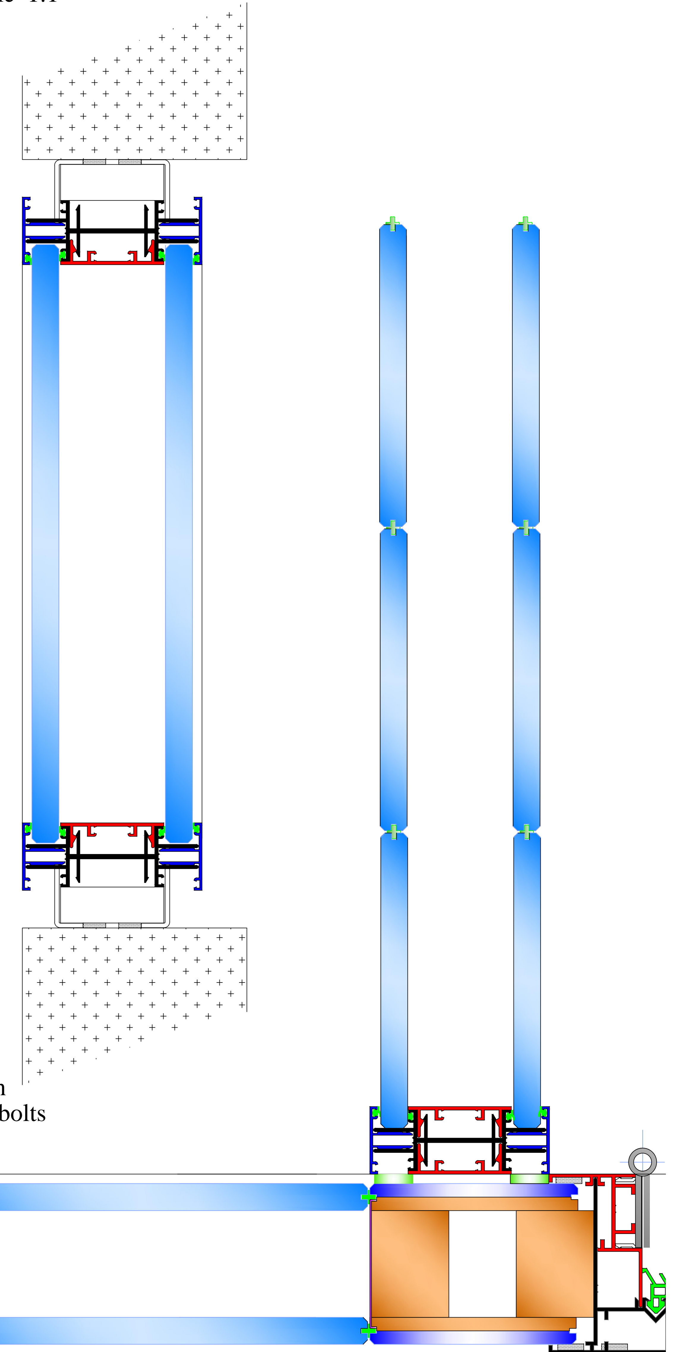
Panels Connection
